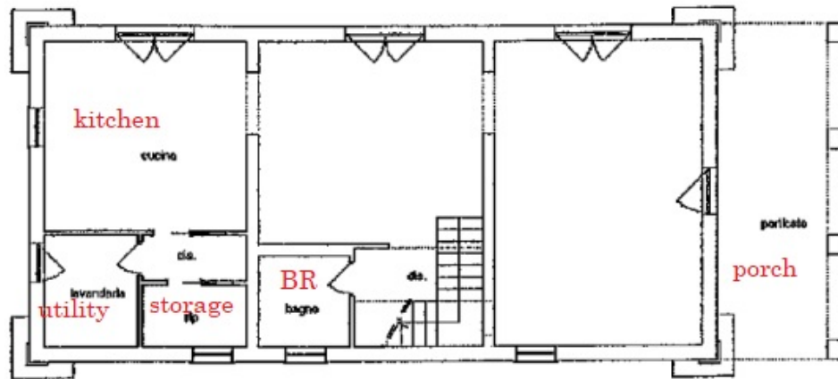
PIANO TERRA GROUND FLOOR h 3.00
