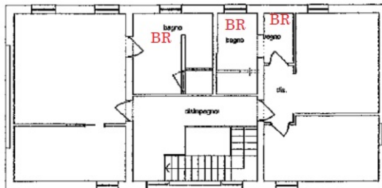
PIANO PRIMO FIRST FLOOR hm 3.20
